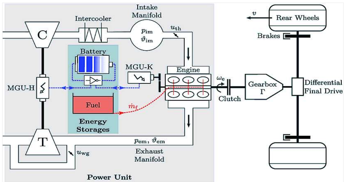
Figure 5: Components of the Formula 1 (F1) hybrid powertrain
