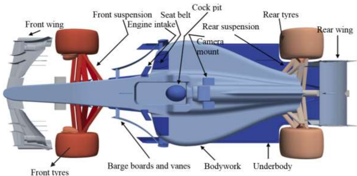
Figure 6: A typical F1 car components
